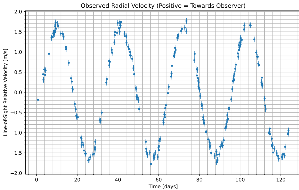
Figure 1: We have isolated the radial velocity of the host star due to the candidate planet. Data begins at UTC 2087-07-12/19:42. Positive values indicate the velocity at which the star is moving towards us; negative indicate the velocity at which it is moving away.
