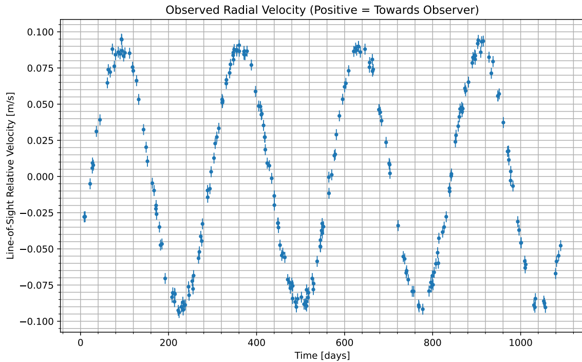
Figure 1: We have isolated the radial velocity of the host star due to the candidate planet. Data begins at UTC 2089-05-16/19:33. Positive values indicate the velocity at which the star is moving towards us; negative indicate the velocity at which it is moving away.
