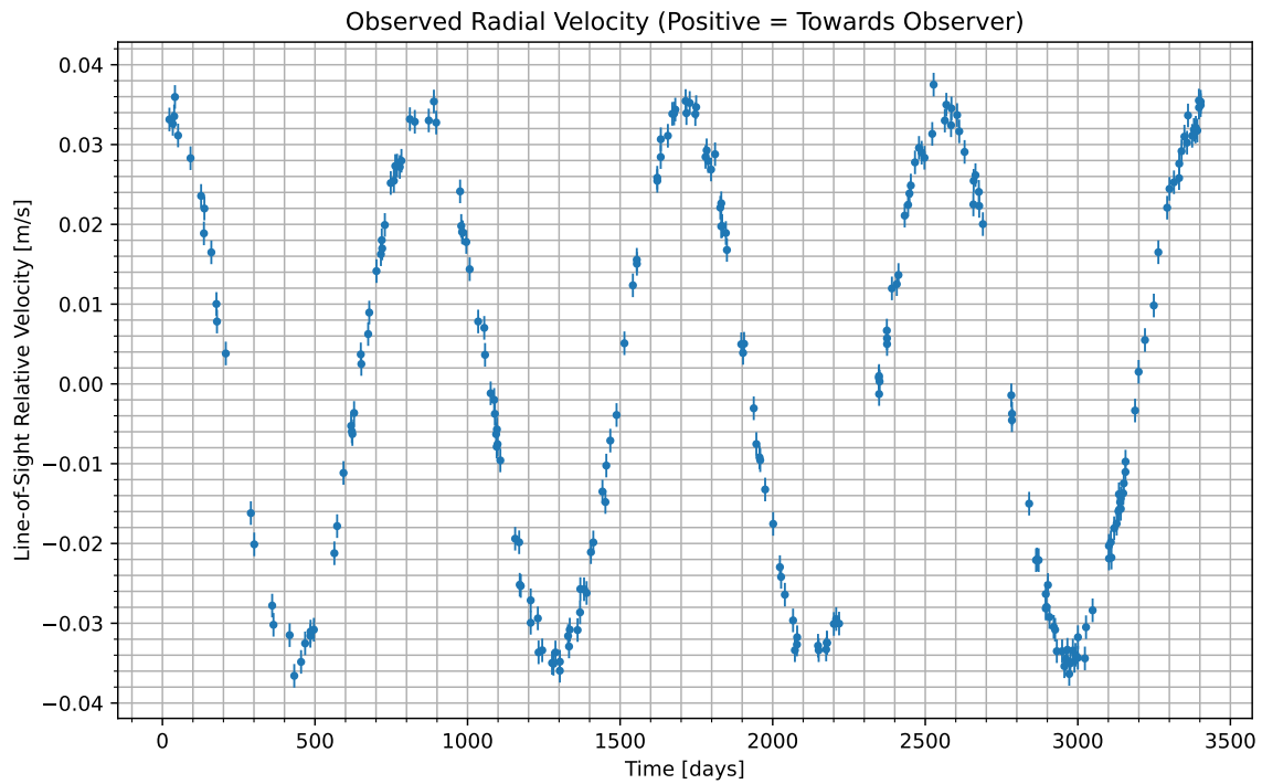
Figure 1: We have isolated the radial velocity of the host star due to the candidate planet. Data begins at UTC 2072-08-20/06:59. Positive values indicate the velocity at which the star is moving towards us; negative indicate the velocity at which it is moving away.
