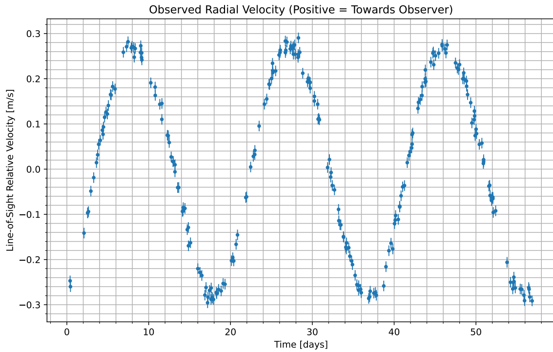
Figure 1: We have isolated the radial velocity of the host star due to the candidate planet. Data begins at UTC 2095-06-28/00:15. Positive values indicate the velocity at which the star is moving towards us; negative indicate the velocity at which it is moving away.
