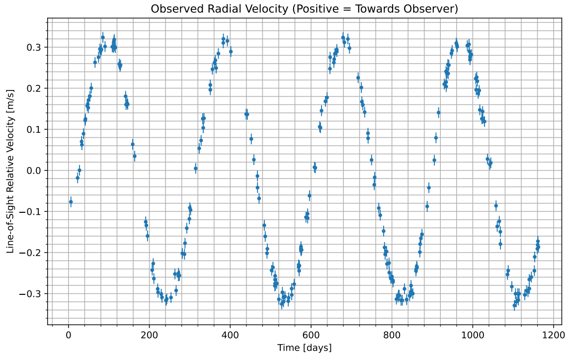
Figure 1: We have isolated the radial velocity of the host star due to the candidate planet. Data begins at UTC 2074-02-24/00:20. Positive values indicate the velocity at which the star is moving towards us; negative indicate the velocity at which it is moving away.
