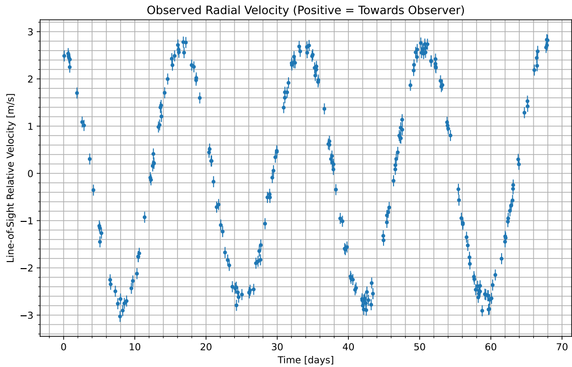
Figure 1: We have isolated the radial velocity of the host star due to the candidate planet. Data begins at UTC 2074-02-11/17:39. Positive values indicate the velocity at which the star is moving towards us; negative indicate the velocity at which it is moving away.
