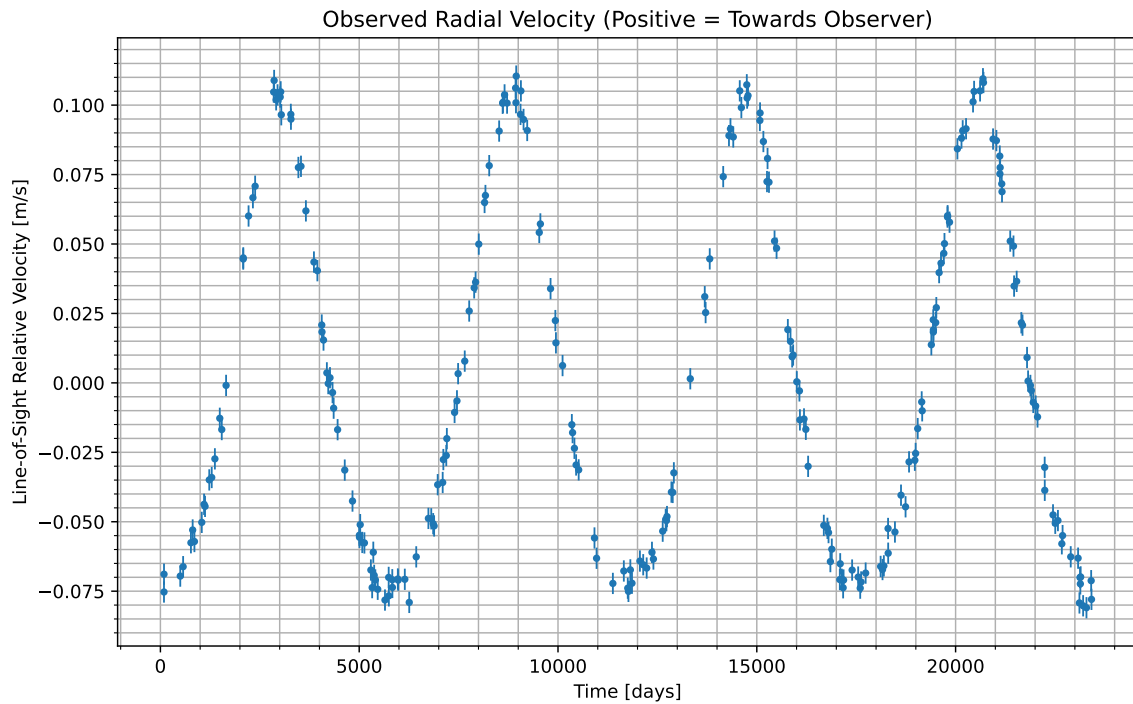
Figure 1: We have isolated the radial velocity of the host star due to the candidate planet. Data begins at UTC 2019-04-12/12:47. Positive values indicate the velocity at which the star is moving towards us; negative indicate the velocity at which it is moving away.
