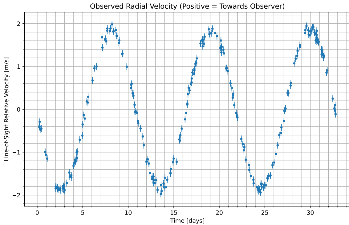
Figure 1: We have isolated the radial velocity of the host star due to the candidate planet. Data begins at UTC 2089-06-09/14:48. Positive values indicate the velocity at which the star is moving towards us; negative indicate the velocity at which it is moving away.
