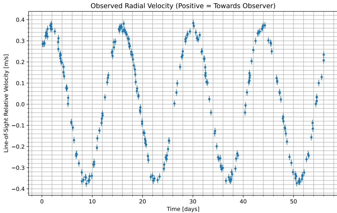
Figure 1: We have isolated the radial velocity of the host star due to the candidate planet. Data begins at UTC 2094-05-19/14:23. Positive values indicate the velocity at which the star is moving towards us; negative indicate the velocity at which it is moving away.
