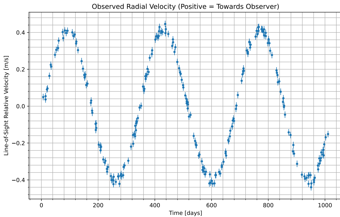
Figure 1: We have isolated the radial velocity of the host star due to the candidate planet. Data begins at UTC 2084-07-10/21:39. Positive values indicate the velocity at which the star is moving towards us; negative indicate the velocity at which it is moving away.
