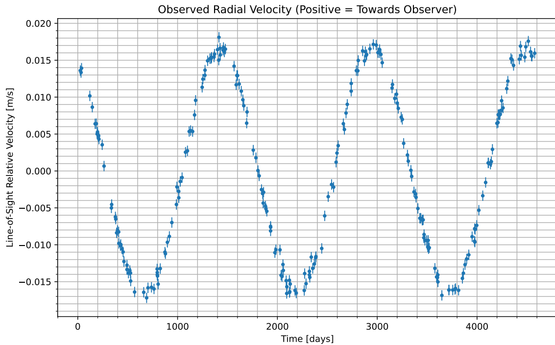
Figure 1: We have isolated the radial velocity of the host star due to the candidate planet. Data begins at UTC 2075-05-22/14:07. Positive values indicate the velocity at which the star is moving towards us; negative indicate the velocity at which it is moving away.
