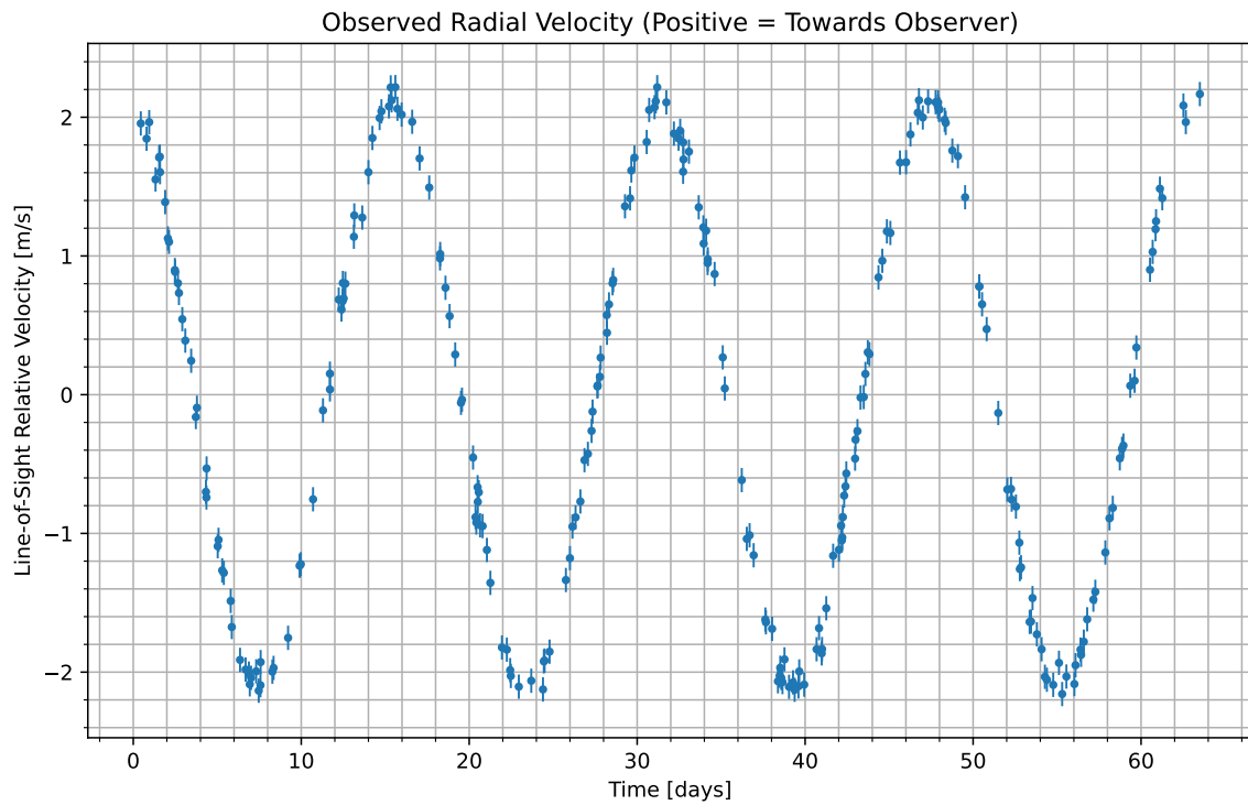
Figure 1: We have isolated the radial velocity of the host star due to the candidate planet. Data begins at UTC 2086-04-22/06:10. Positive values indicate the velocity at which the star is moving towards us; negative indicate the velocity at which it is moving away.
