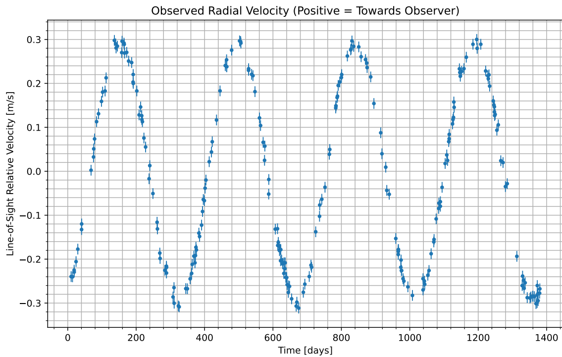
Figure 1: We have isolated the radial velocity of the host star due to the candidate planet. Data begins at UTC 2096-06-18/07:03. Positive values indicate the velocity at which the star is moving towards us; negative indicate the velocity at which it is moving away.
