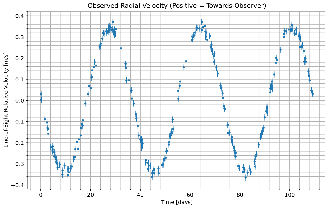
Figure 1: We have isolated the radial velocity of the host star due to the candidate planet. Data begins at UTC 2084-11-10/14:11. Positive values indicate the velocity at which the star is moving towards us; negative indicate the velocity at which it is moving away.
