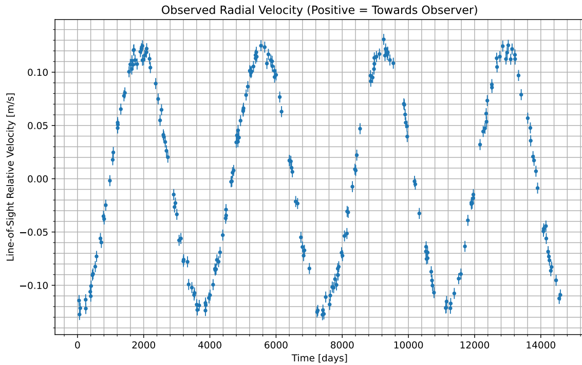
Figure 1: We have isolated the radial velocity of the host star due to the candidate planet. Data begins at UTC 2037-06-24/08:44. Positive values indicate the velocity at which the star is moving towards us; negative indicate the velocity at which it is moving away.
