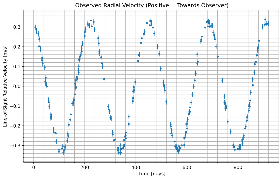
Figure 1: We have isolated the radial velocity of the host star due to the candidate planet. Data begins at UTC 2074-09-23/12:43. Positive values indicate the velocity at which the star is moving towards us; negative indicate the velocity at which it is moving away.
