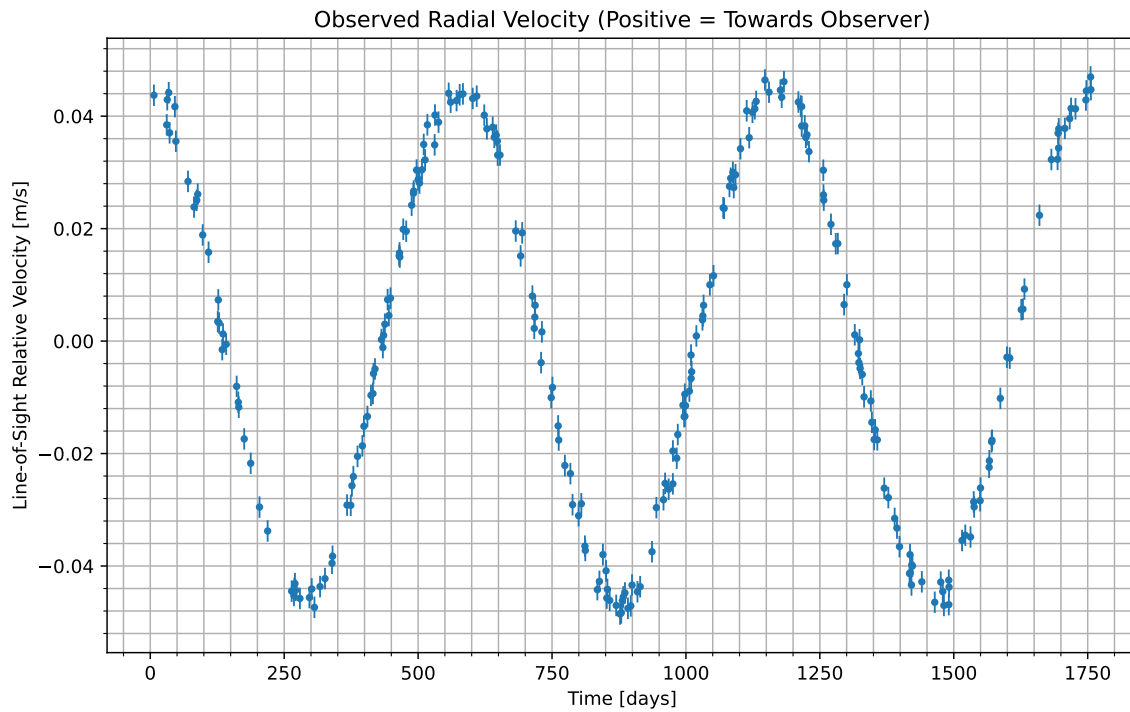
Figure 1: We have isolated the radial velocity of the host star due to the candidate planet. Data begins at UTC 2070-03-18/19:04. Positive values indicate the velocity at which the star is moving towards us; negative indicate the velocity at which it is moving away.
