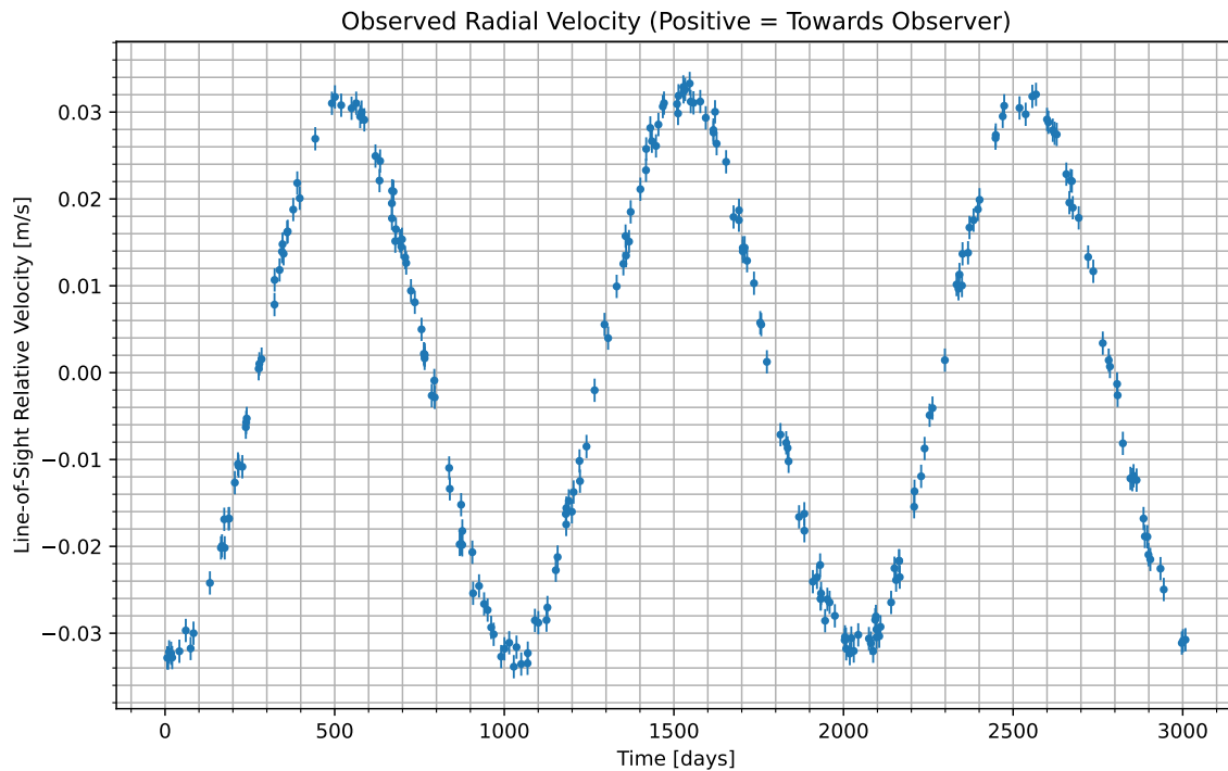
Figure 1: We have isolated the radial velocity of the host star due to the candidate planet. Data begins at UTC 2063-01-31/16:20. Positive values indicate the velocity at which the star is moving towards us; negative indicate the velocity at which it is moving away.
