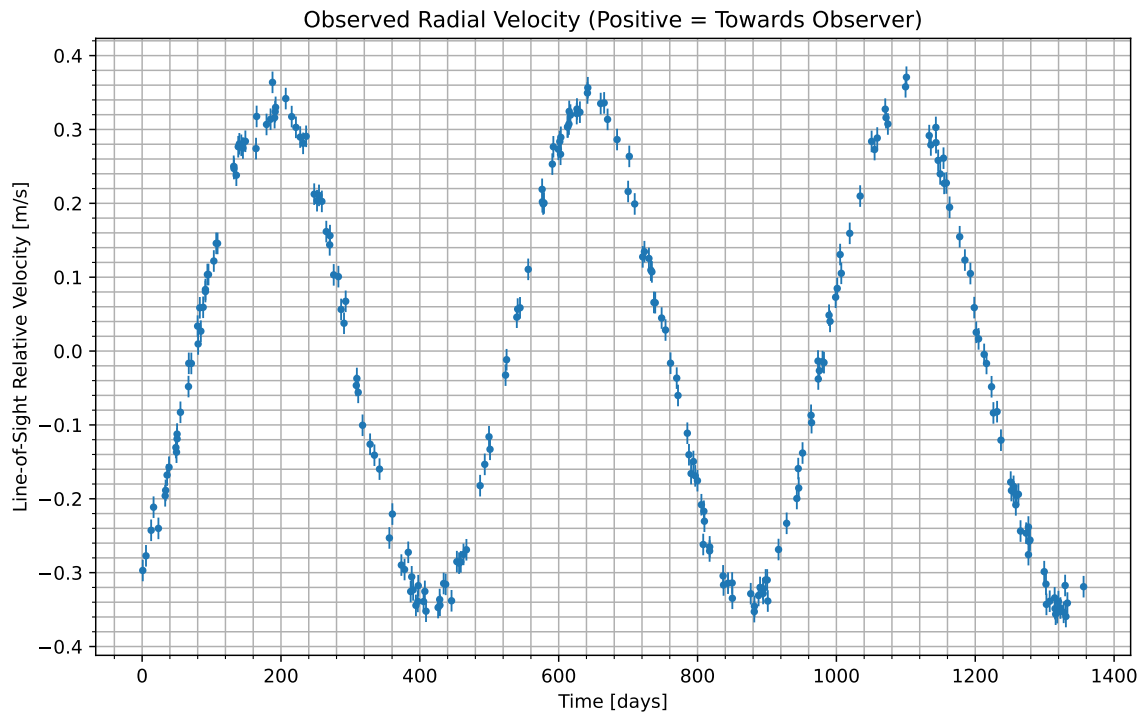
Figure 1: We have isolated the radial velocity of the host star due to the candidate planet. Data begins at UTC 2072-10-19/14:00. Positive values indicate the velocity at which the star is moving towards us; negative indicate the velocity at which it is moving away.
