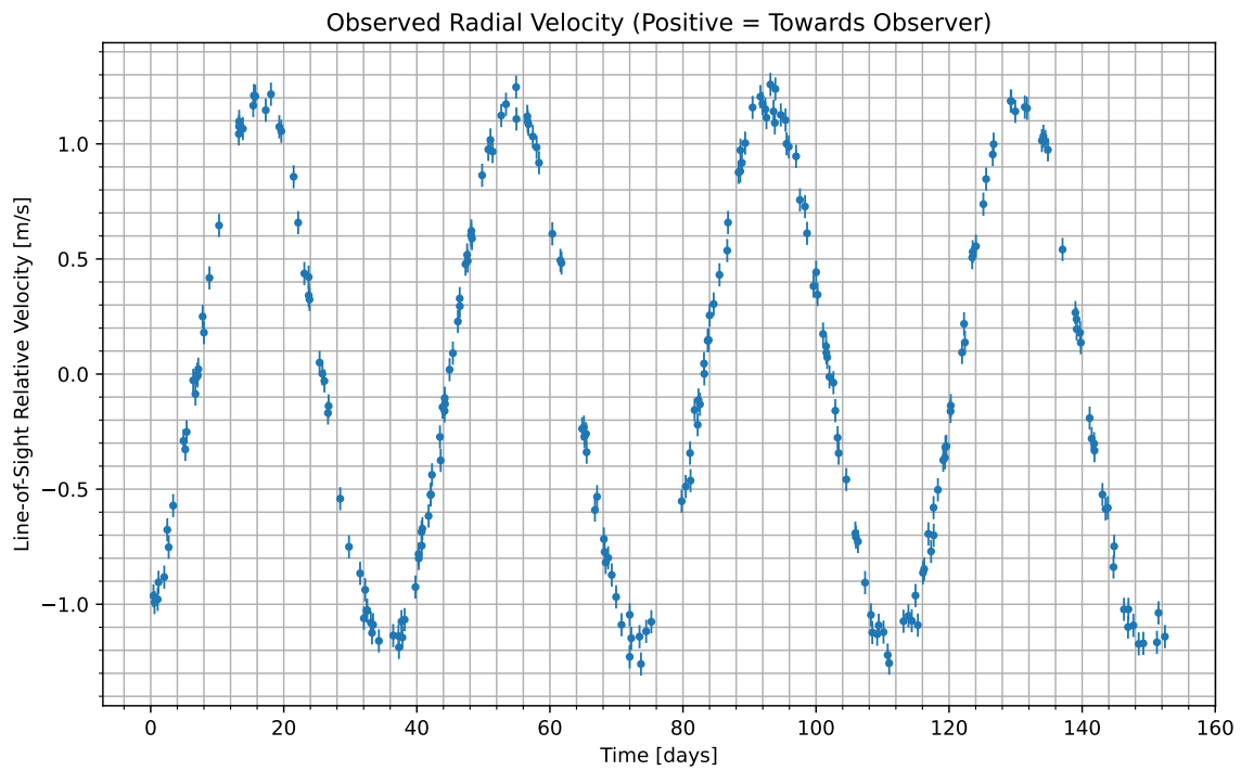
Figure 1: We have isolated the radial velocity of the host star due to the candidate planet. Data begins at UTC 2093-02-15/11:46. Positive values indicate the velocity at which the star is moving towards us; negative indicate the velocity at which it is moving away.
