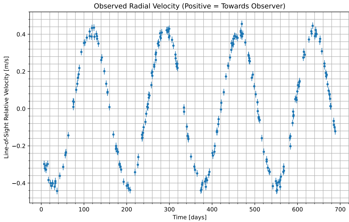
Figure 1: We have isolated the radial velocity of the host star due to the candidate planet. Data begins at UTC 2077-10-30/20:46. Positive values indicate the velocity at which the star is moving towards us; negative indicate the velocity at which it is moving away.
