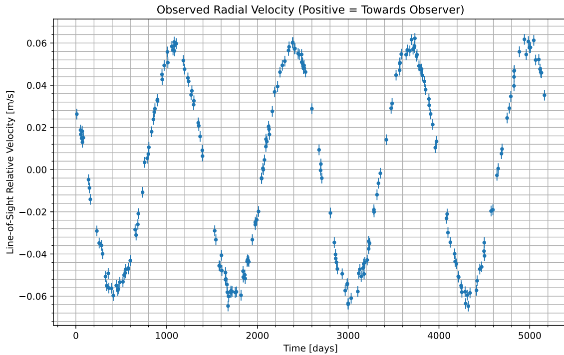
Figure 1: We have isolated the radial velocity of the host star due to the candidate planet. Data begins at UTC 2068-07-15/10:39. Positive values indicate the velocity at which the star is moving towards us; negative indicate the velocity at which it is moving away.
