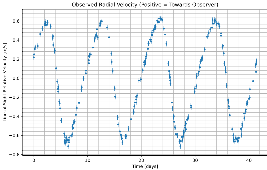
Figure 1: We have isolated the radial velocity of the host star due to the candidate planet. Data begins at UTC 2100-08-12/10:52. Positive values indicate the velocity at which the star is moving towards us; negative indicate the velocity at which it is moving away.
