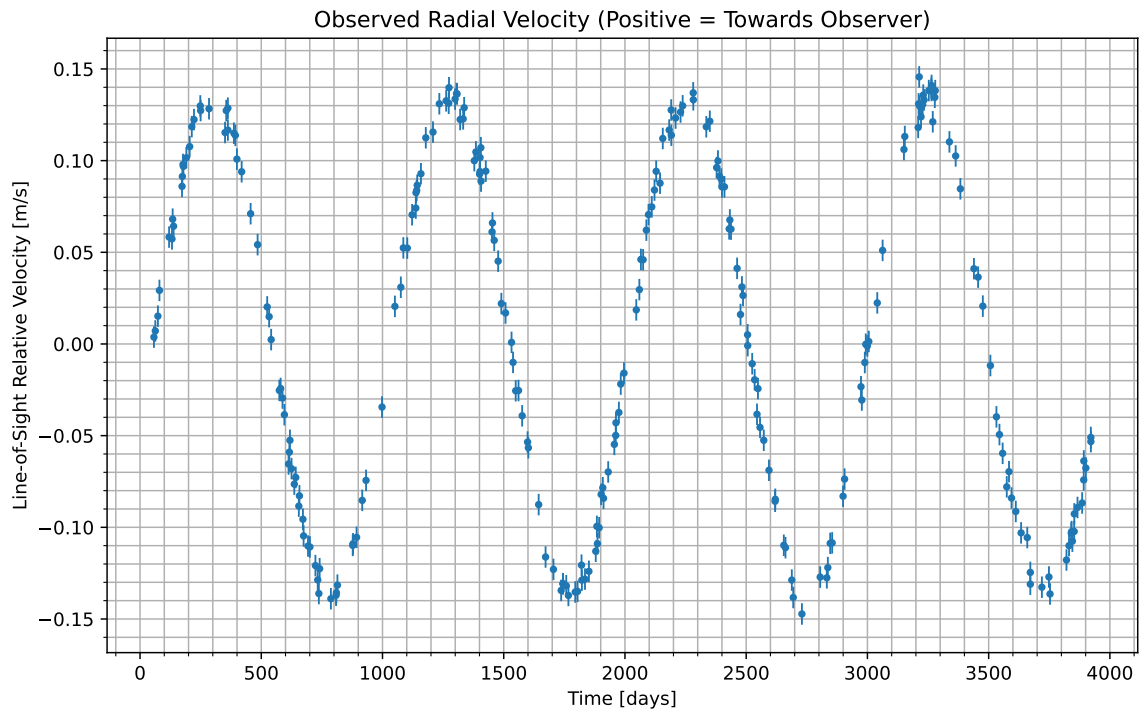
Figure 1: We have isolated the radial velocity of the host star due to the candidate planet. Data begins at UTC 2064-02-04/18:34. Positive values indicate the velocity at which the star is moving towards us; negative indicate the velocity at which it is moving away.
