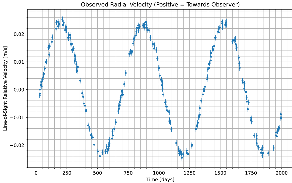
Figure 1: We have isolated the radial velocity of the host star due to the candidate planet. Data begins at UTC 2073-07-16/10:32. Positive values indicate the velocity at which the star is moving towards us; negative indicate the velocity at which it is moving away.
