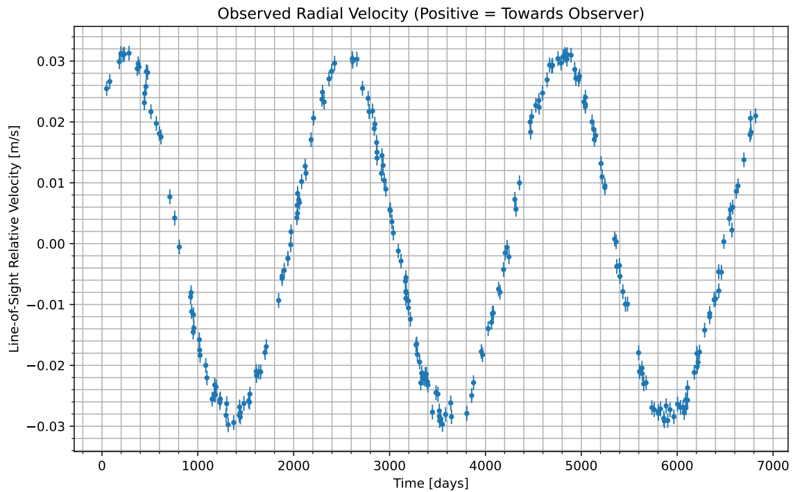
Figure 1: We have isolated the radial velocity of the host star due to the candidate planet. Data begins at UTC 2071-02-21/06:20. Positive values indicate the velocity at which the star is moving towards us; negative indicate the velocity at which it is moving away.
