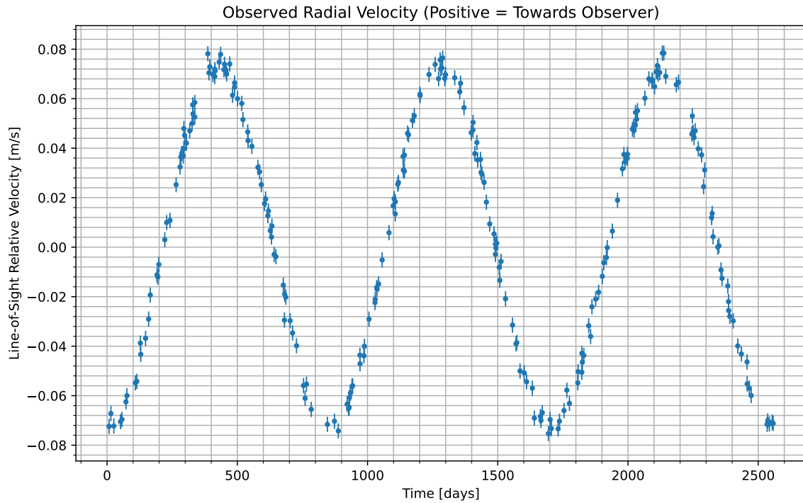
Figure 1: We have isolated the radial velocity of the host star due to the candidate planet. Data begins at UTC 2069-07-24/20:22. Positive values indicate the velocity at which the star is moving towards us; negative indicate the velocity at which it is moving away.
