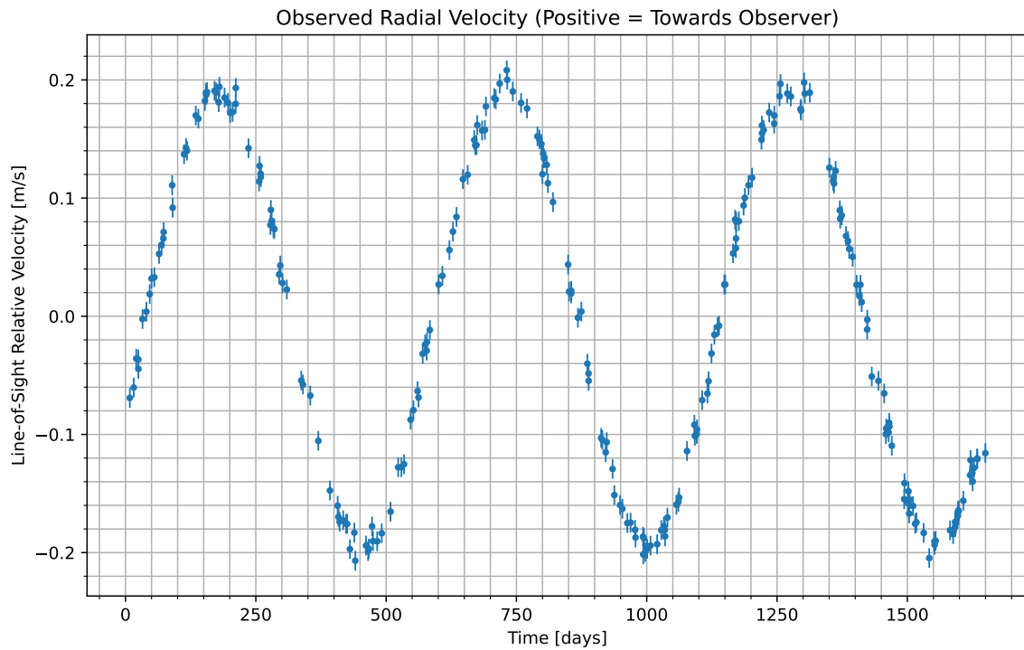
Figure 1: We have isolated the radial velocity of the host star due to the candidate planet. Data begins at UTC 2075-11-15/04:53. Positive values indicate the velocity at which the star is moving towards us; negative indicate the velocity at which it is moving away.
