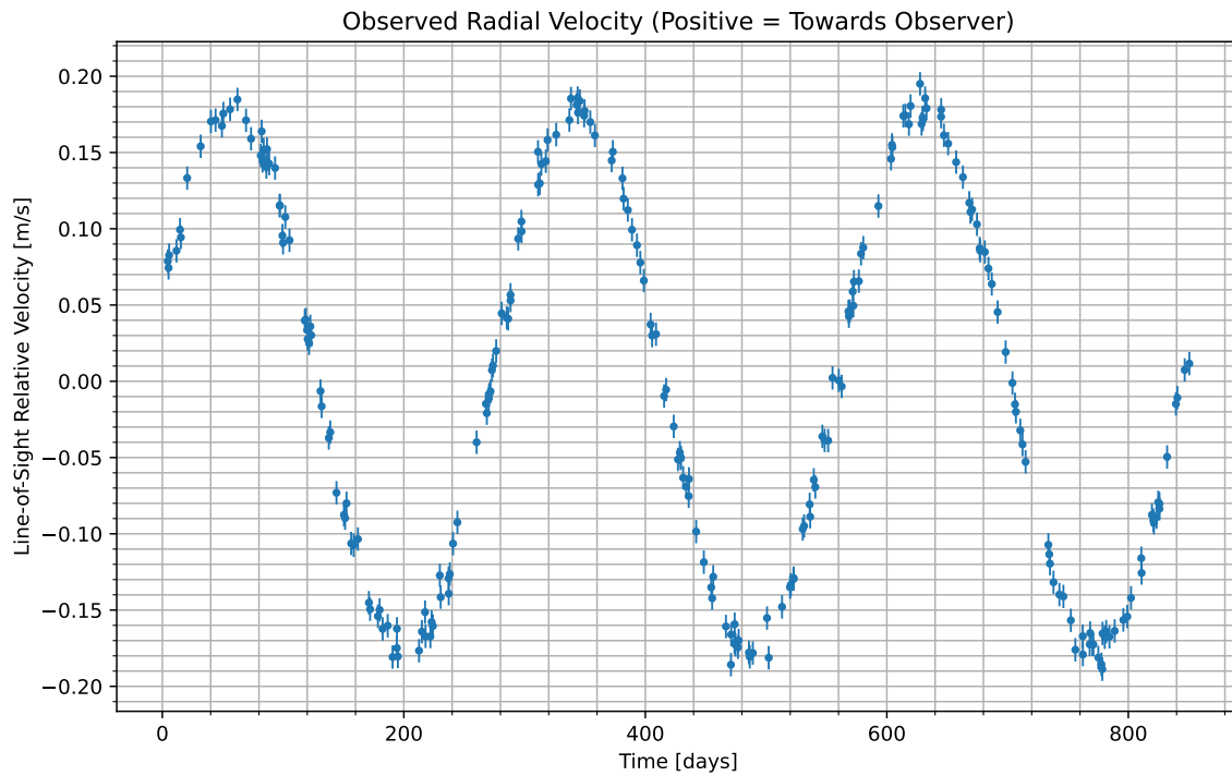
Figure 1: We have isolated the radial velocity of the host star due to the candidate planet. Data begins at UTC 2080-10-15/10:15. Positive values indicate the velocity at which the star is moving towards us; negative indicate the velocity at which it is moving away.
