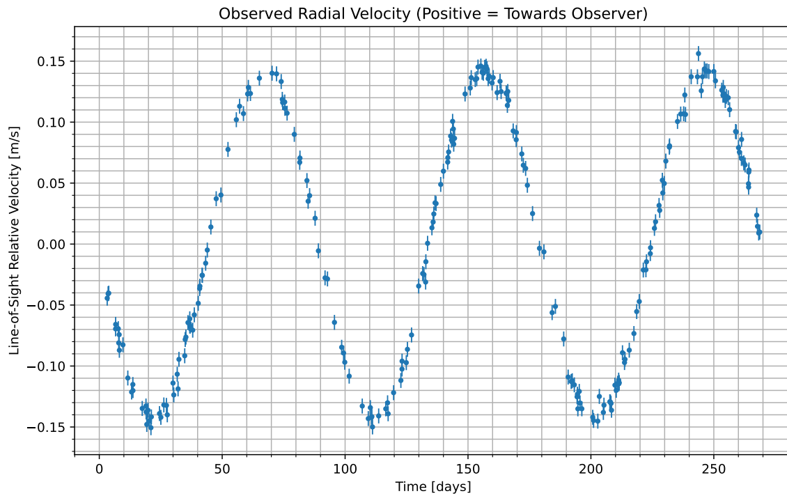
Figure 1: We have isolated the radial velocity of the host star due to the candidate planet. Data begins at UTC 2090-10-11/13:22. Positive values indicate the velocity at which the star is moving towards us; negative indicate the velocity at which it is moving away.
