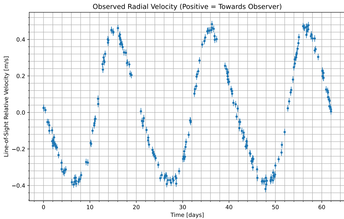
Figure 1: We have isolated the radial velocity of the host star due to the candidate planet. Data begins at UTC 2093-08-21/08:42. Positive values indicate the velocity at which the star is moving towards us; negative indicate the velocity at which it is moving away.
