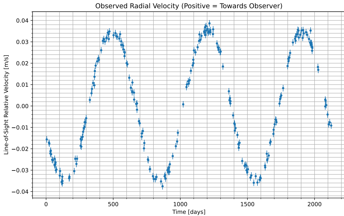
Figure 1: We have isolated the radial velocity of the host star due to the candidate planet. Data begins at UTC 2076-10-31/13:18. Positive values indicate the velocity at which the star is moving towards us; negative indicate the velocity at which it is moving away.
