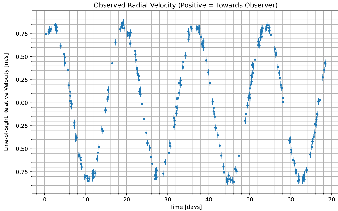
Figure 1: We have isolated the radial velocity of the host star due to the candidate planet. Data begins at UTC 2079-07-21/06:45. Positive values indicate the velocity at which the star is moving towards us; negative indicate the velocity at which it is moving away.
