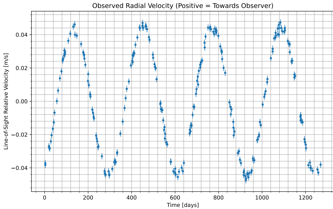
Figure 1: We have isolated the radial velocity of the host star due to the candidate planet. Data begins at UTC 2080-05-11/22:51. Positive values indicate the velocity at which the star is moving towards us; negative indicate the velocity at which it is moving away.
