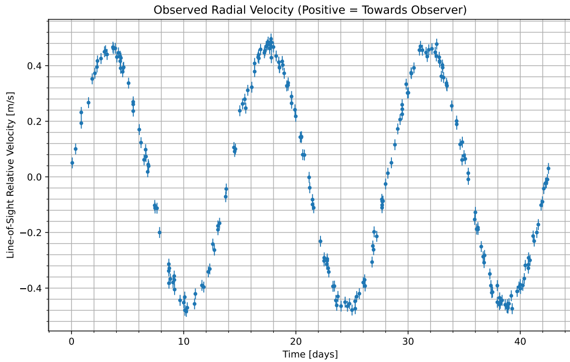
Figure 1: We have isolated the radial velocity of the host star due to the candidate planet. Data begins at UTC 2079-01-29/22:02. Positive values indicate the velocity at which the star is moving towards us; negative indicate the velocity at which it is moving away.
