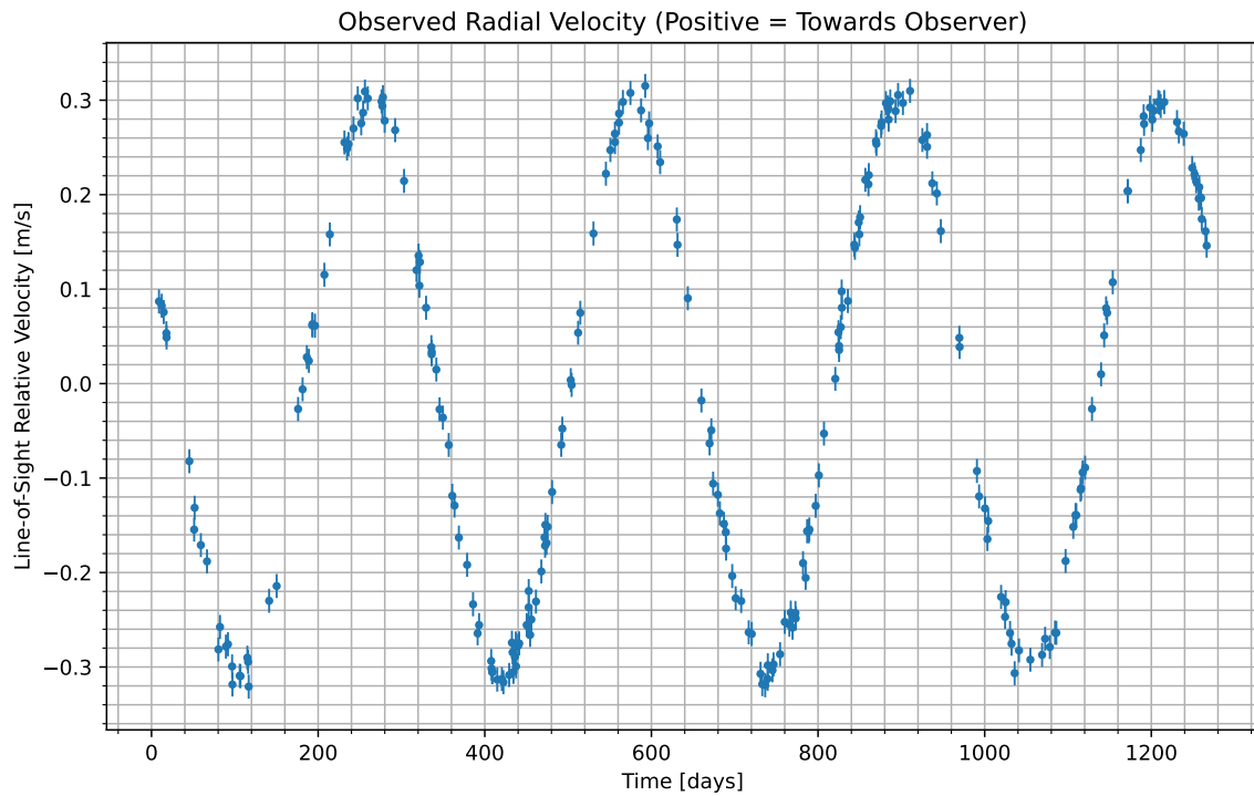
Figure 1: We have isolated the radial velocity of the host star due to the candidate planet. Data begins at UTC 2073-02-19/03:44. Positive values indicate the velocity at which the star is moving towards us; negative indicate the velocity at which it is moving away.
