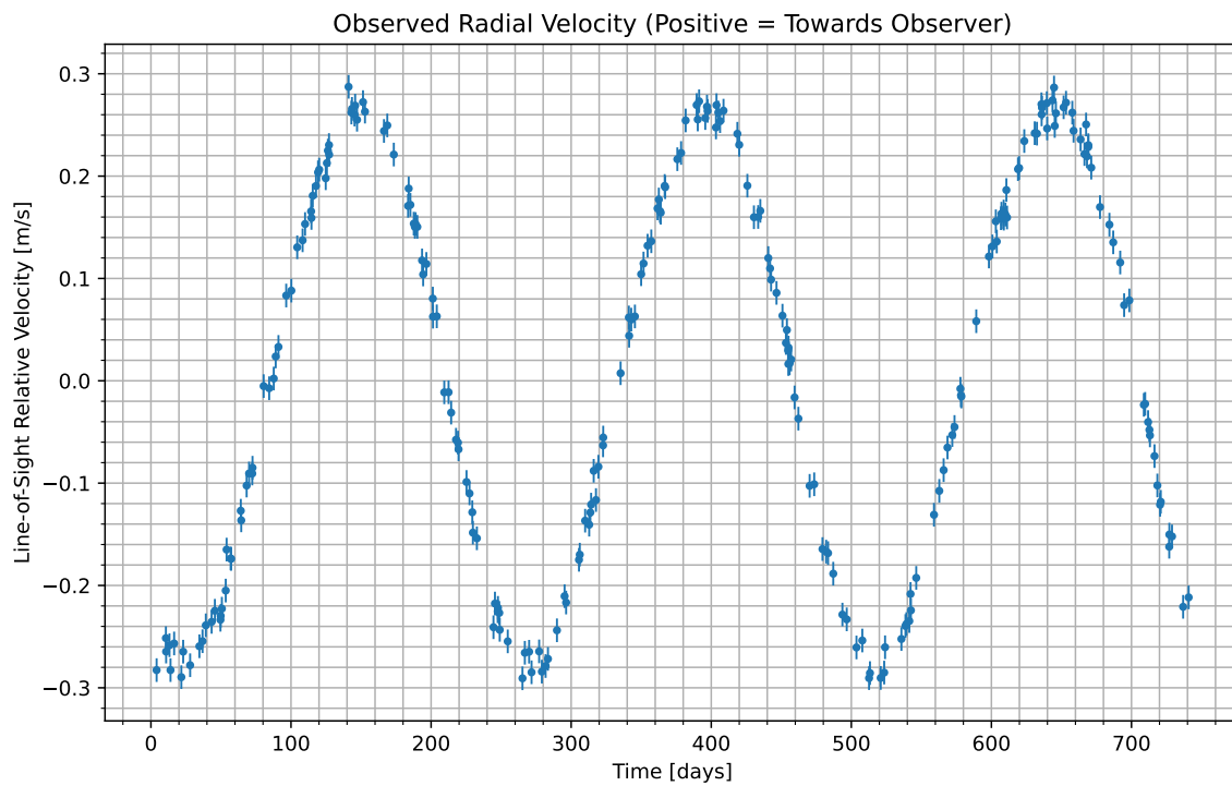
Figure 1: We have isolated the radial velocity of the host star due to the candidate planet. Data begins at UTC 2081-08-27/01:30. Positive values indicate the velocity at which the star is moving towards us; negative indicate the velocity at which it is moving away.
