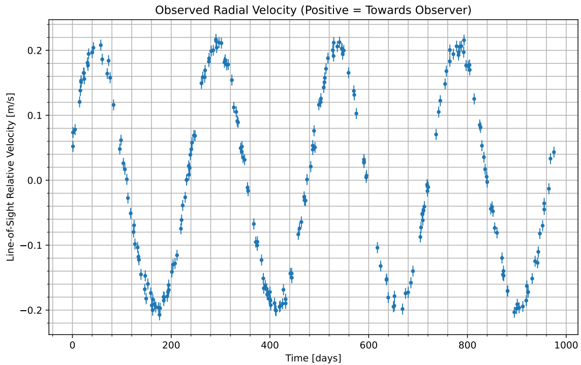
Figure 1: We have isolated the radial velocity of the host star due to the candidate planet. Data begins at UTC 2090-06-11/23:03. Positive values indicate the velocity at which the star is moving towards us; negative indicate the velocity at which it is moving away.
