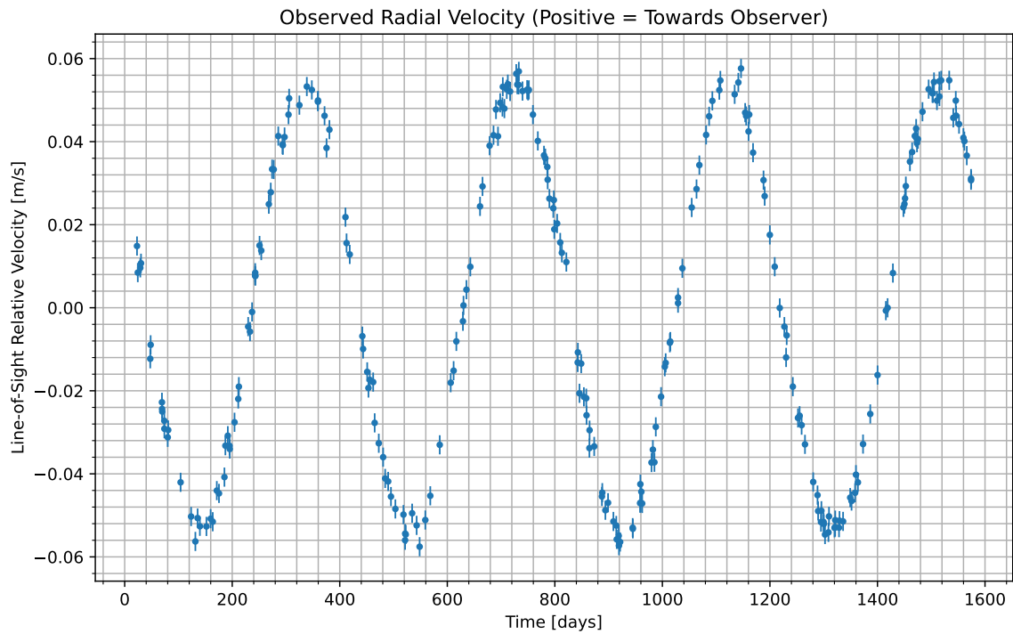
Figure 1: We have isolated the radial velocity of the host star due to the candidate planet. Data begins at UTC 2075-02-28/06:36. Positive values indicate the velocity at which the star is moving towards us; negative indicate the velocity at which it is moving away.
