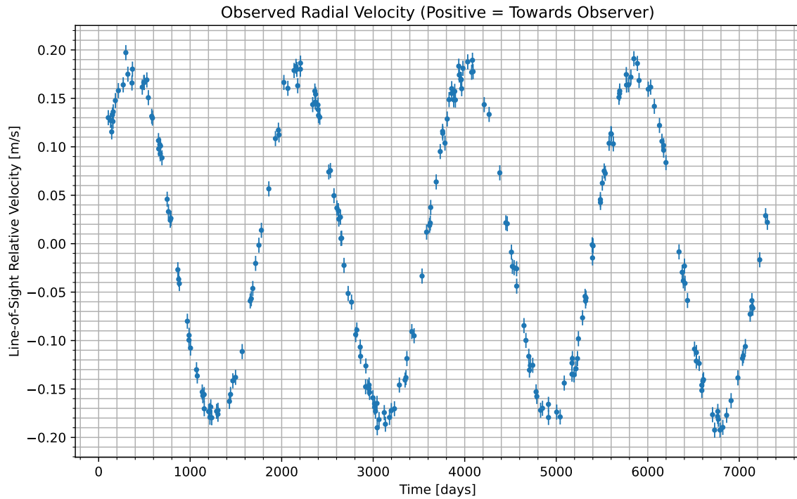
Figure 1: We have isolated the radial velocity of the host star due to the candidate planet. Data begins at UTC 2060-02-18/12:40. Positive values indicate the velocity at which the star is moving towards us; negative indicate the velocity at which it is moving away.
