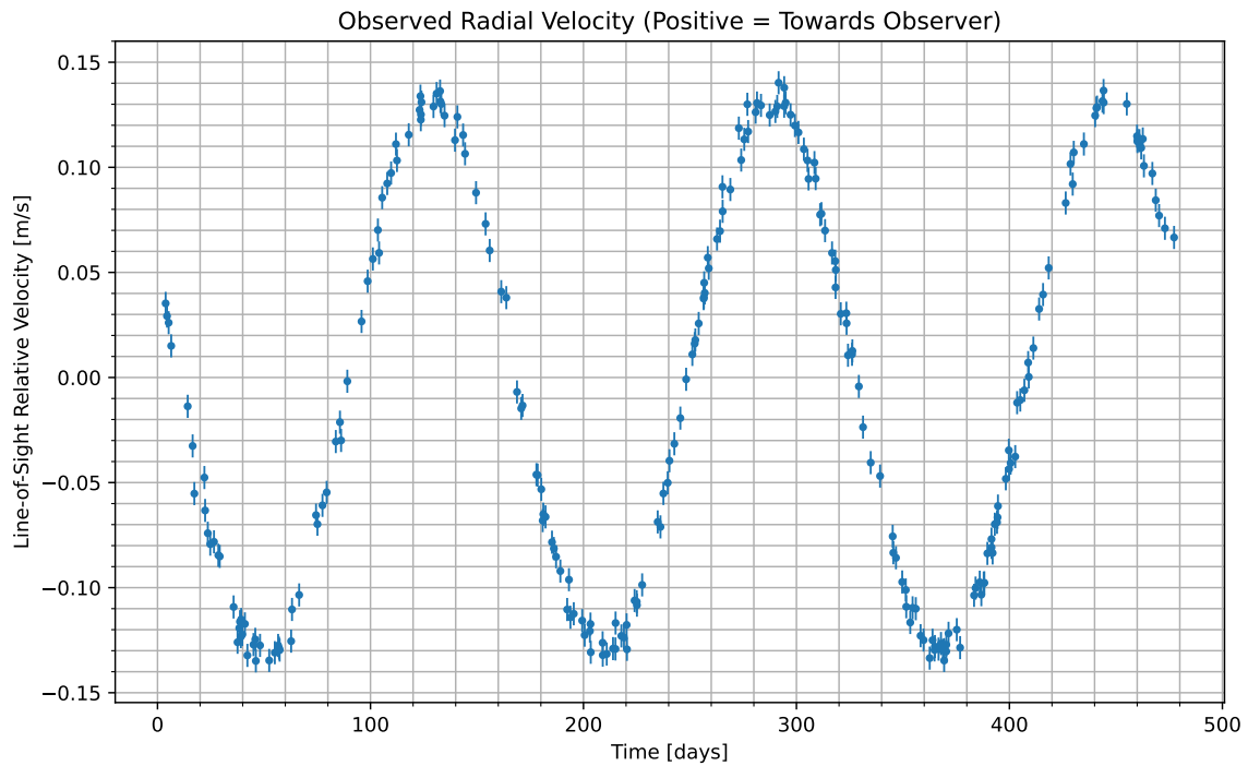
Figure 1: We have isolated the radial velocity of the host star due to the candidate planet. Data begins at UTC 2074-10-01/07:25. Positive values indicate the velocity at which the star is moving towards us; negative indicate the velocity at which it is moving away.
