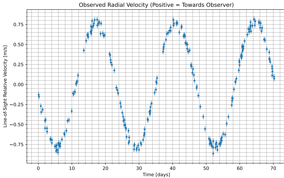
Figure 1: We have isolated the radial velocity of the host star due to the candidate planet. Data begins at UTC 2092-05-26/11:33. Positive values indicate the velocity at which the star is moving towards us; negative indicate the velocity at which it is moving away.
