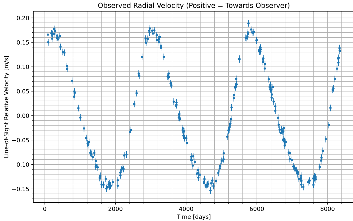
Figure 1: We have isolated the radial velocity of the host star due to the candidate planet. Data begins at UTC 2056-06-21/13:17. Positive values indicate the velocity at which the star is moving towards us; negative indicate the velocity at which it is moving away.
