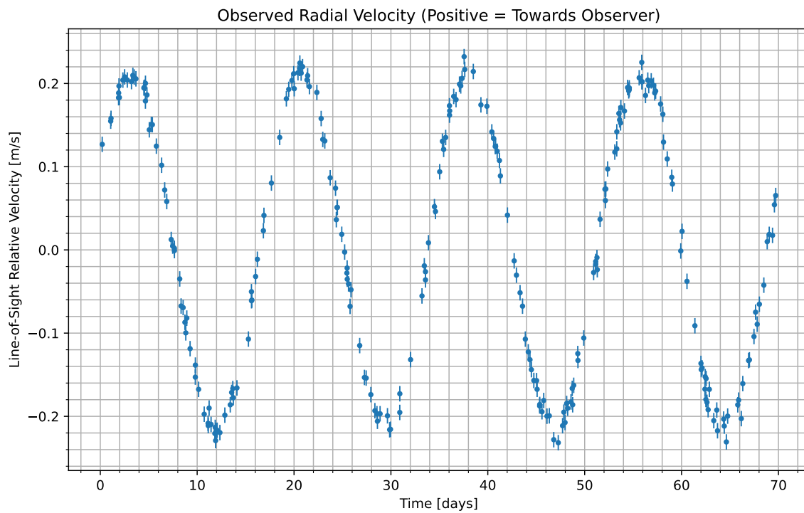
Figure 1: We have isolated the radial velocity of the host star due to the candidate planet. Data begins at UTC 2083-12-12/01:03. Positive values indicate the velocity at which the star is moving towards us; negative indicate the velocity at which it is moving away.
