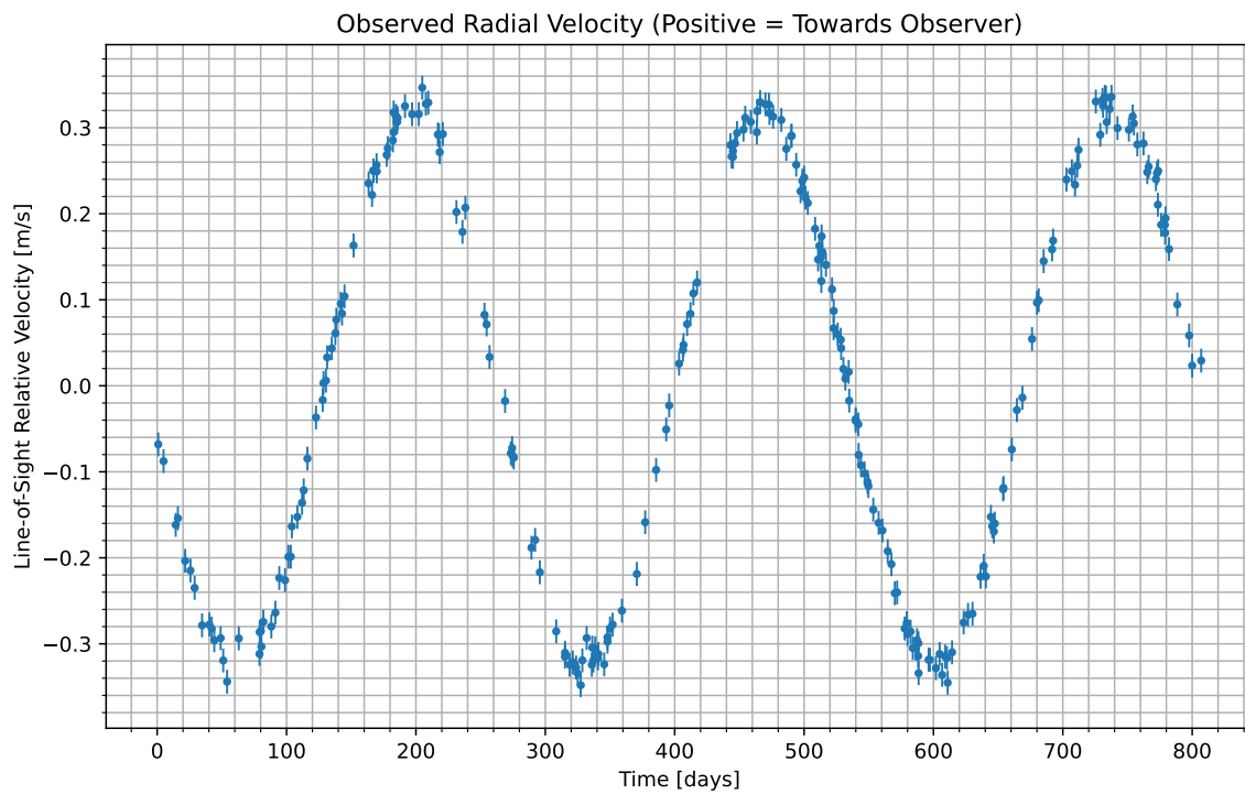
Figure 1: We have isolated the radial velocity of the host star due to the candidate planet. Data begins at UTC 2073-10-12/21:12. Positive values indicate the velocity at which the star is moving towards us; negative indicate the velocity at which it is moving away.
