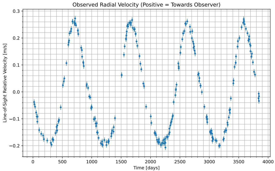
Figure 1: We have isolated the radial velocity of the host star due to the candidate planet. Data begins at UTC 2066-11-05/03:22. Positive values indicate the velocity at which the star is moving towards us; negative indicate the velocity at which it is moving away.
