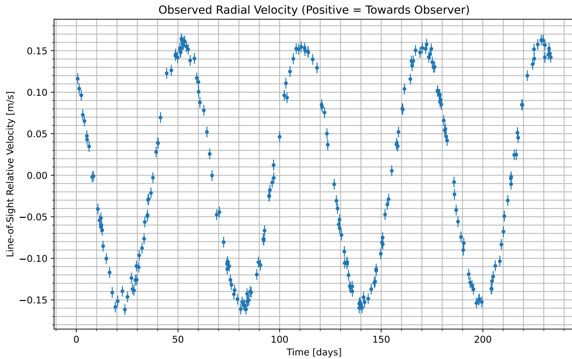
Figure 1: We have isolated the radial velocity of the host star due to the candidate planet. Data begins at UTC 2090-01-23/15:29. Positive values indicate the velocity at which the star is moving towards us; negative indicate the velocity at which it is moving away.
