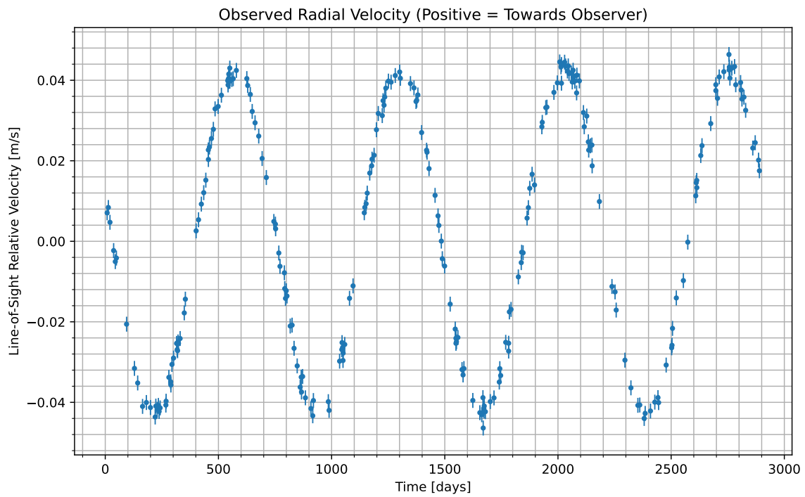
Figure 1: We have isolated the radial velocity of the host star due to the candidate planet. Data begins at UTC 2066-09-29/18:43. Positive values indicate the velocity at which the star is moving towards us; negative indicate the velocity at which it is moving away.
