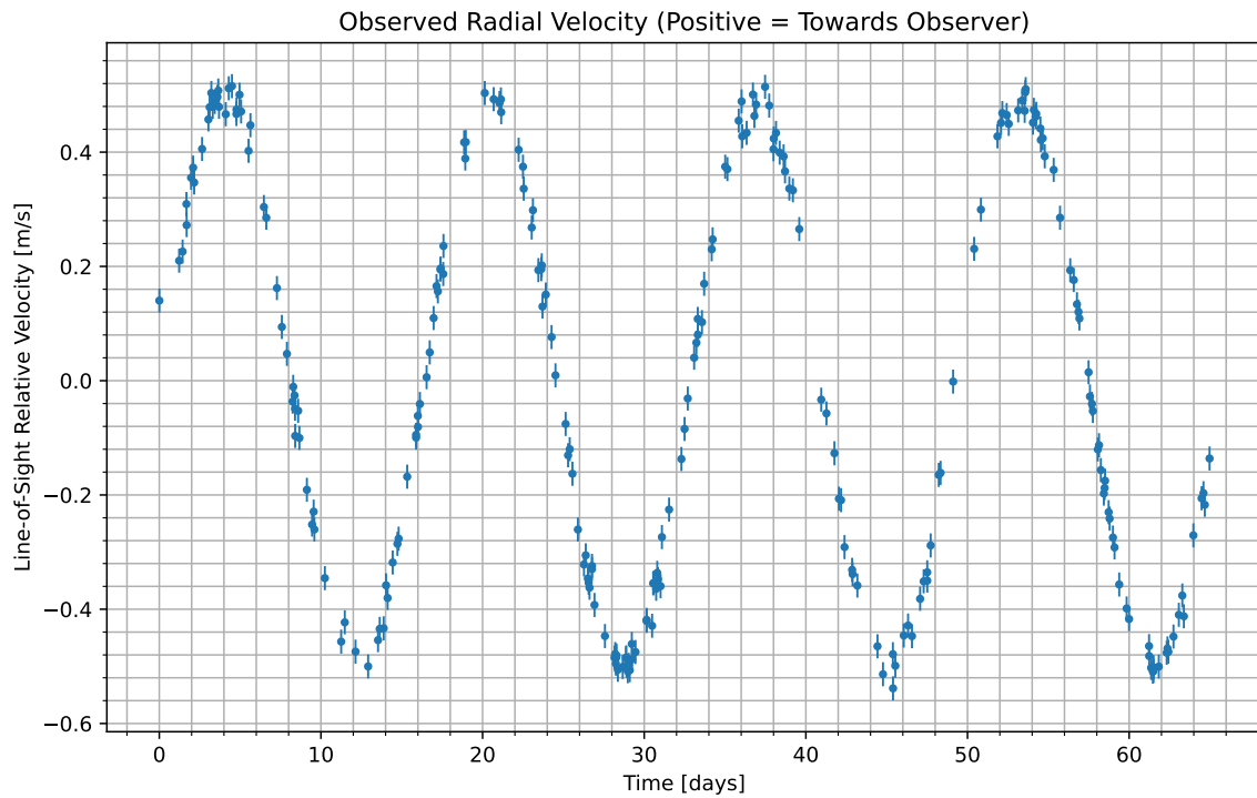
Figure 1: We have isolated the radial velocity of the host star due to the candidate planet. Data begins at UTC 2083-08-05/23:54. Positive values indicate the velocity at which the star is moving towards us; negative indicate the velocity at which it is moving away.
