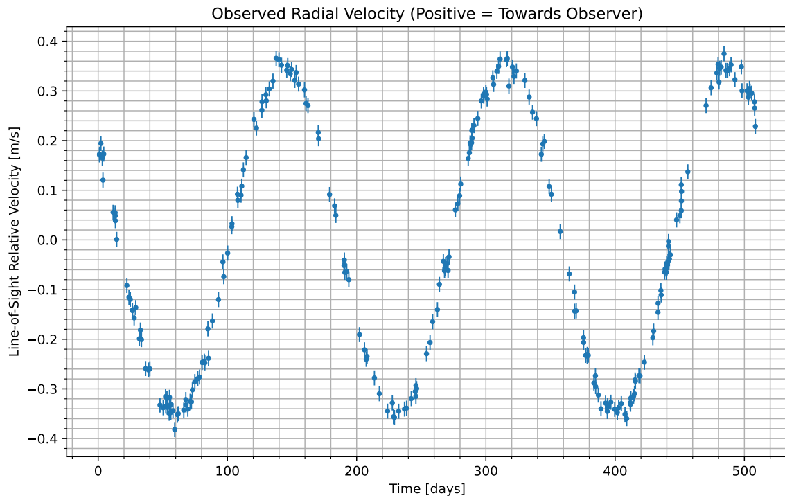
Figure 1: We have isolated the radial velocity of the host star due to the candidate planet. Data begins at UTC 2092-03-31/03:08. Positive values indicate the velocity at which the star is moving towards us; negative indicate the velocity at which it is moving away.
